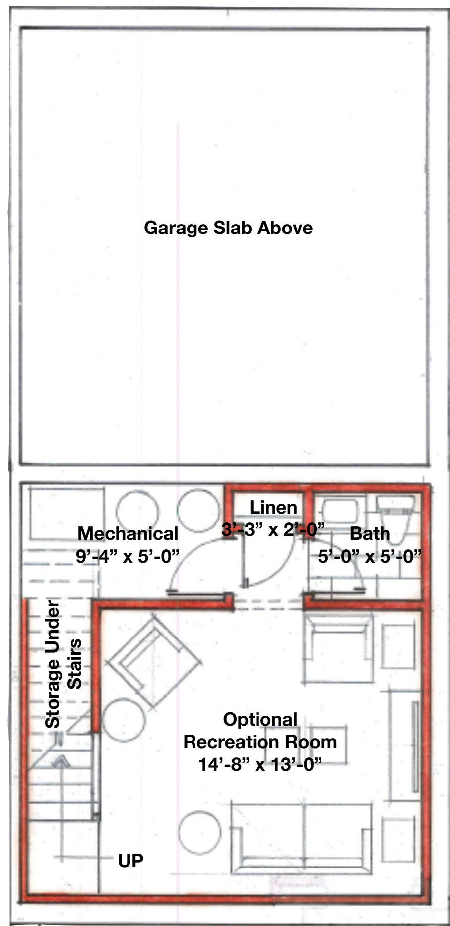
Lower Level 420 square feet
